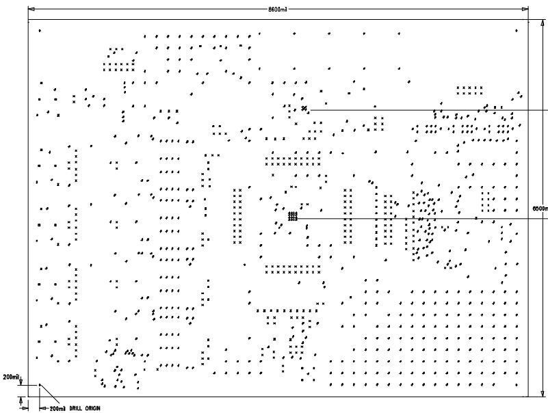
Figure 18. EVAL-ADAU1977Z Fabrication Drawing
