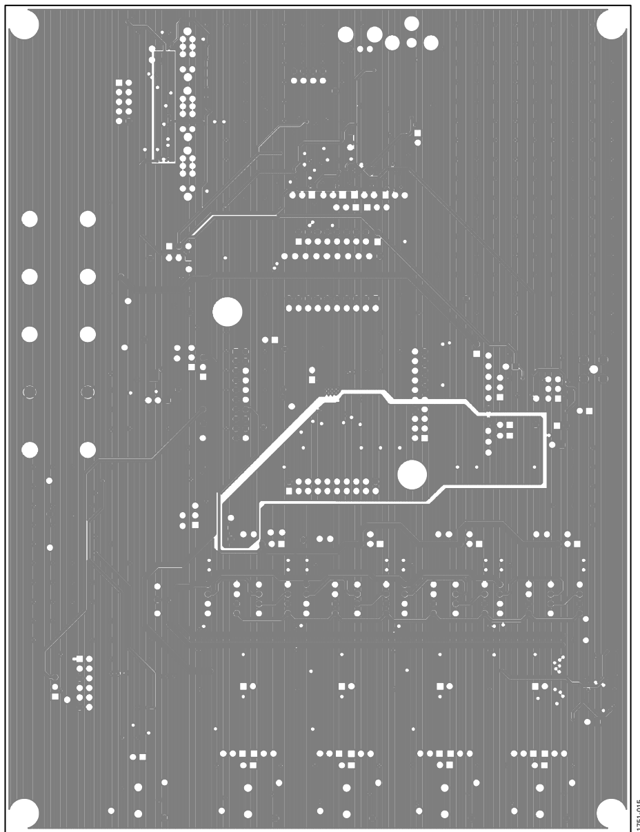
Figure 15. EVAL-ADAU1977Z Layer 3
