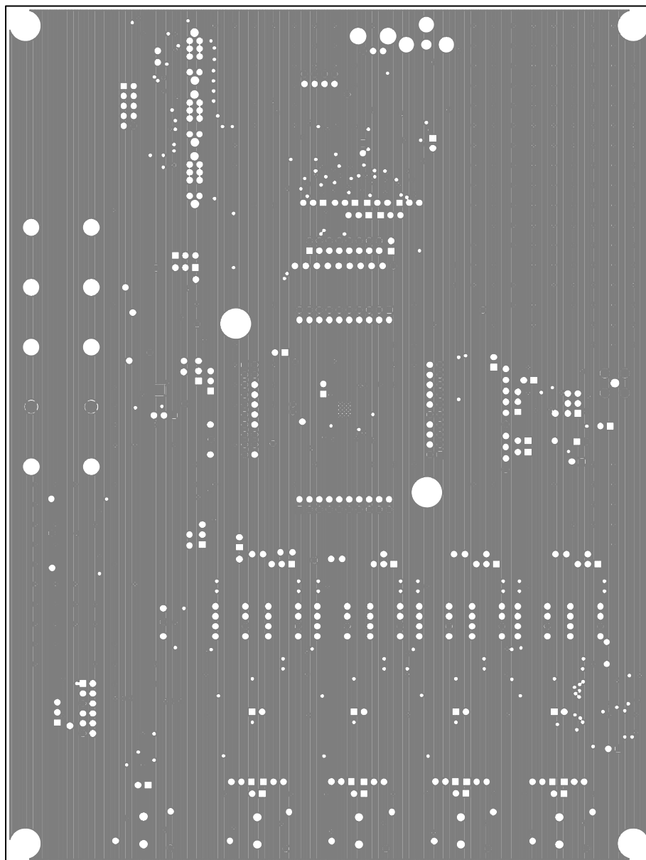
Figure 14. EVAL-ADAU1977Z Layer 2
