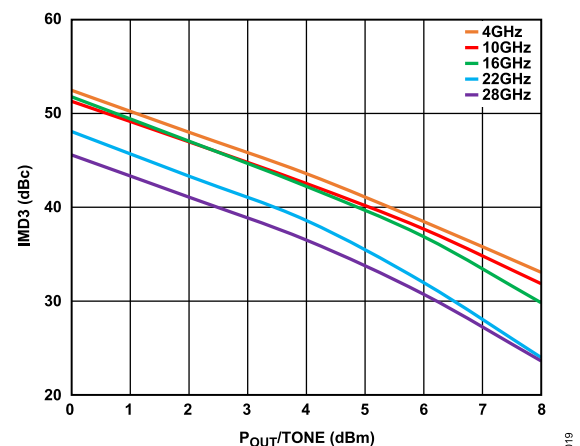
Figure 19. Output Third-Order Intermodulation Distortion ( IMD_3 ) vs. P_{OUT}/Tone at Various Frequencies, V_{DD} = 4 V
