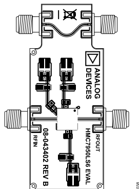
Figure 40. Evaluation PCB
