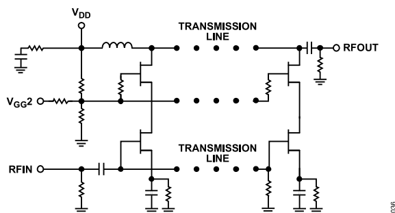
Figure 38. Architecture and Simplified Schematic
