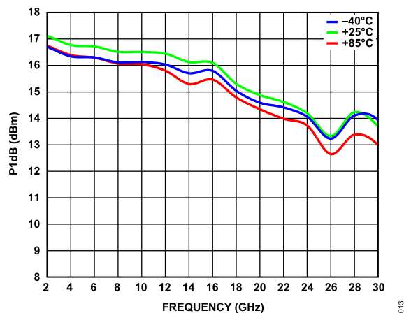
Figure 13. P1dB vs. Frequency at Various Temperatures
