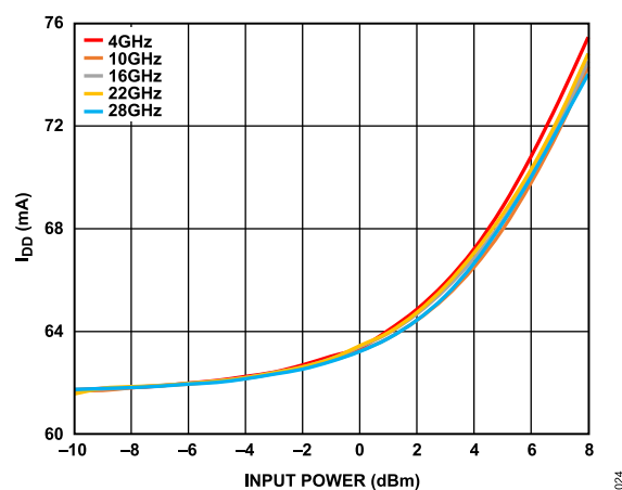
Figure 24. I_{DD} vs. Input Power at Various Frequencies
