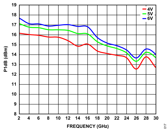
Figure 17. P_{1dB} vs. Frequency at Various Supply Voltages
