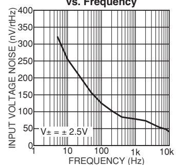
MIC863 Input Voltage Noise vs. Frequency
