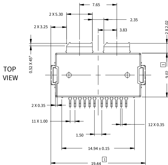
Package PG-HB1DSO-14-4
