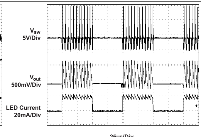
Figure 19. PWM Dimming
