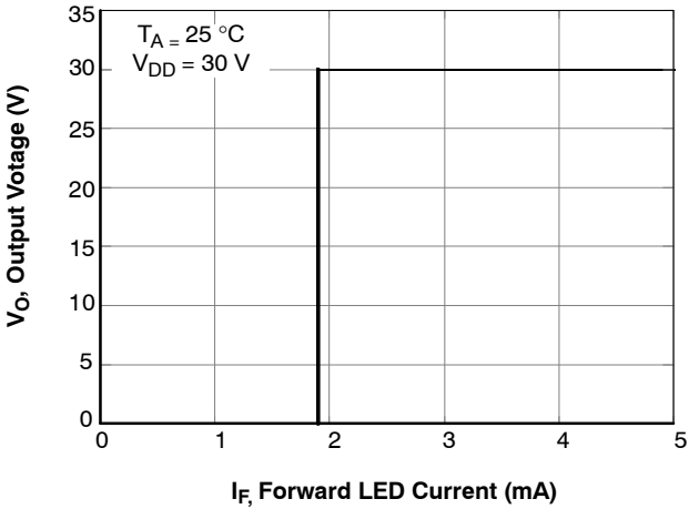
Figure 13. Transfer Characteristics
