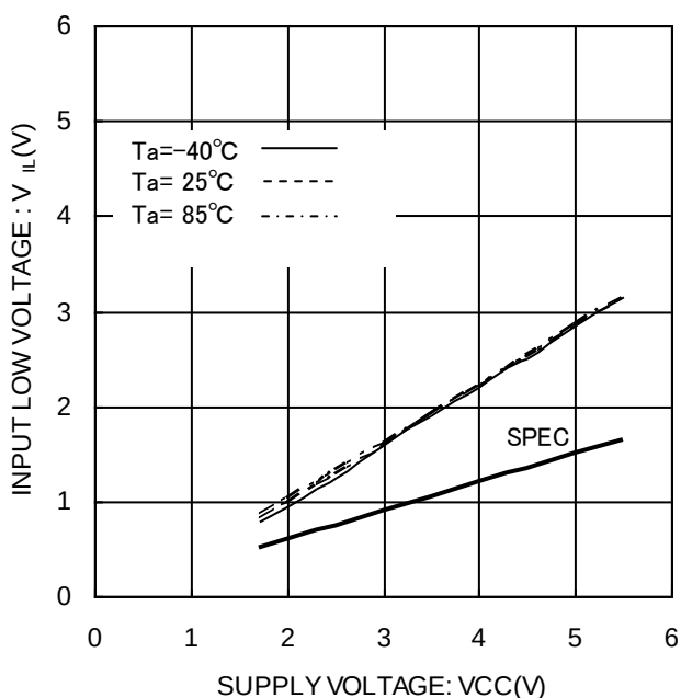
Figure 5. Input low voltage V_{IL} (CS,SK,DI,ORG)
