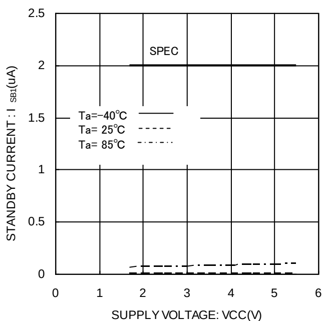
Figure 19. Standby current I_{SBI}(CS=0V, \text{ORG}=VCC \text{ or } \text{OPEN})
