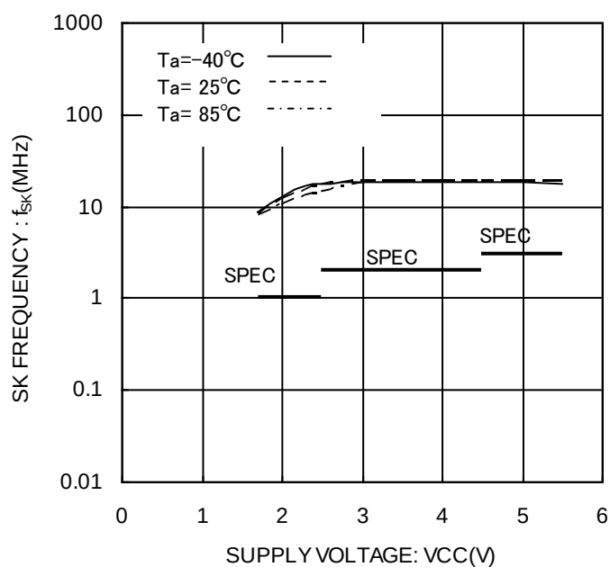
Figure 21. SK frequency f_{SK}
