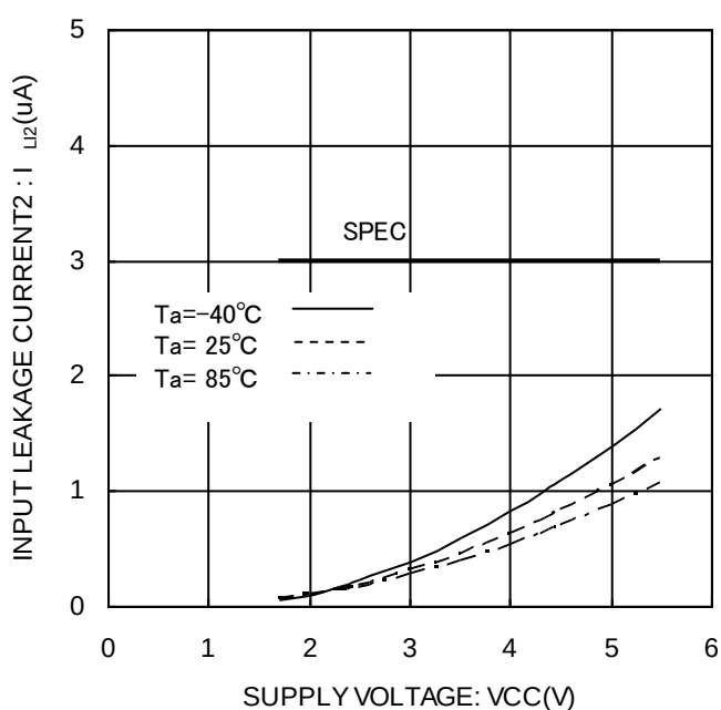
Figure 11. Input leakage current2 I_{LI2}(ORG)
