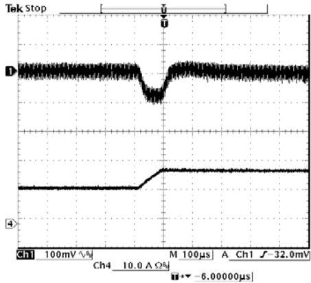
Vout= 3.3 V 50%-75% Load Transients at Vin=48 V
