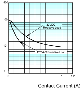
ENDURANCE CURVE
