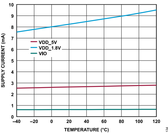
Figure 35. Supply Current vs. Temperature, AD4630-24, 2 MSPS
