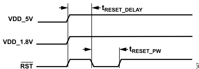
Figure 47. Power-On Reset (POR) Timing
