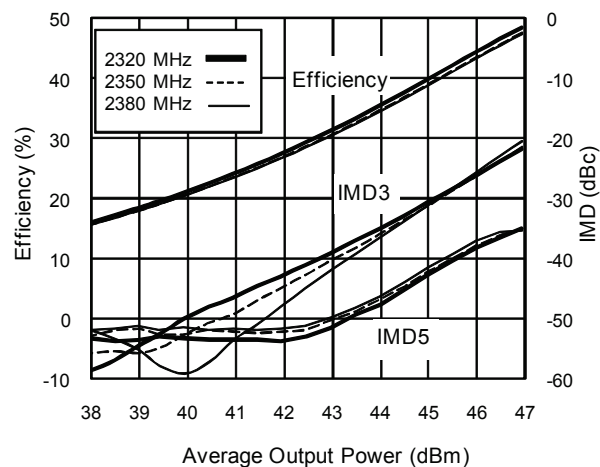
Two-tone Performance at Selected Frequencies, Single Side V_{DD} = 30\text{ V} , I_{DQ} = 660\text{ mA} , 1 MHz Spacing
