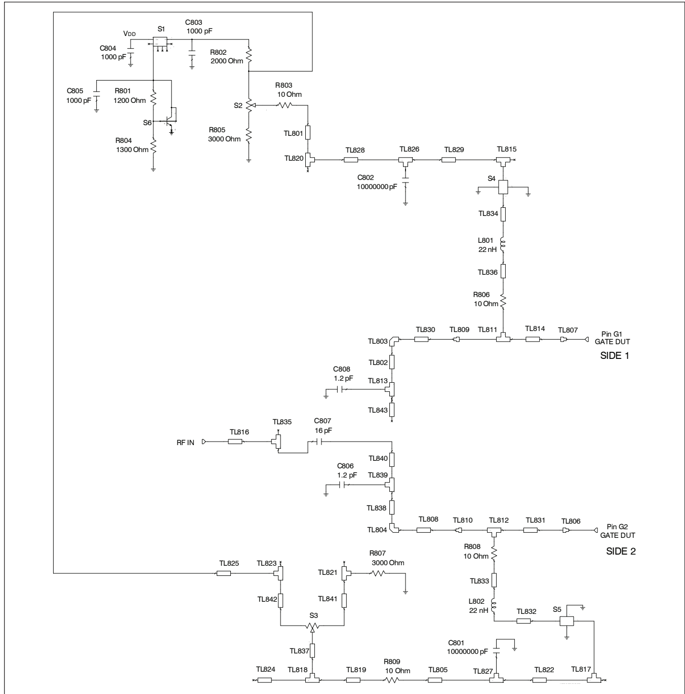
Reference circuit input schematic for f = 2380 MHz
