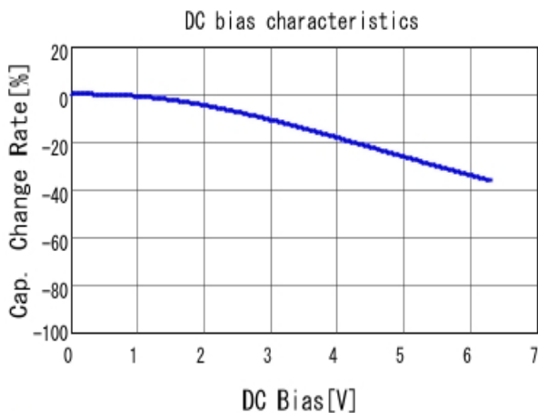
■ GRM32DR60J226MA01 C-DC bias capchange, 25.0degC, AC0.
