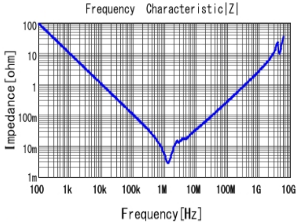
■ GRM32DR60J226MA01 |Z| DC0V, 25degC
