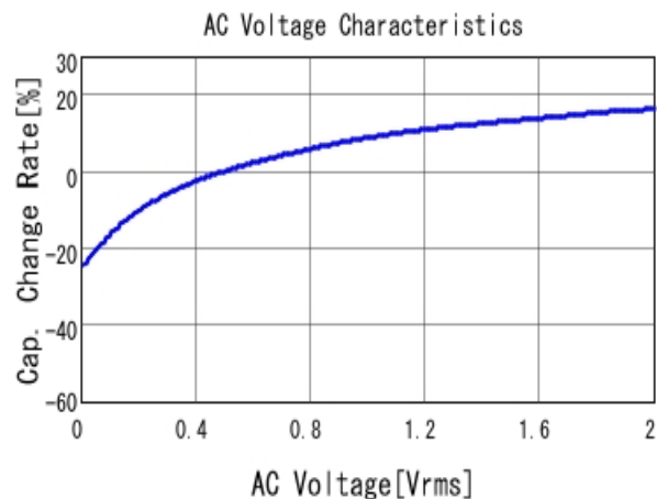
■ GRM32DR60J226MA01 C-AC Voltage capchange, DC0V, 25.0d
