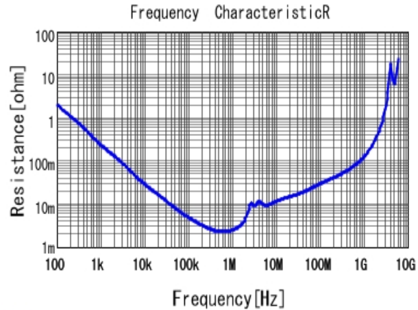
■ GRM32DR60J226MA01 R DC0V, 25degC
