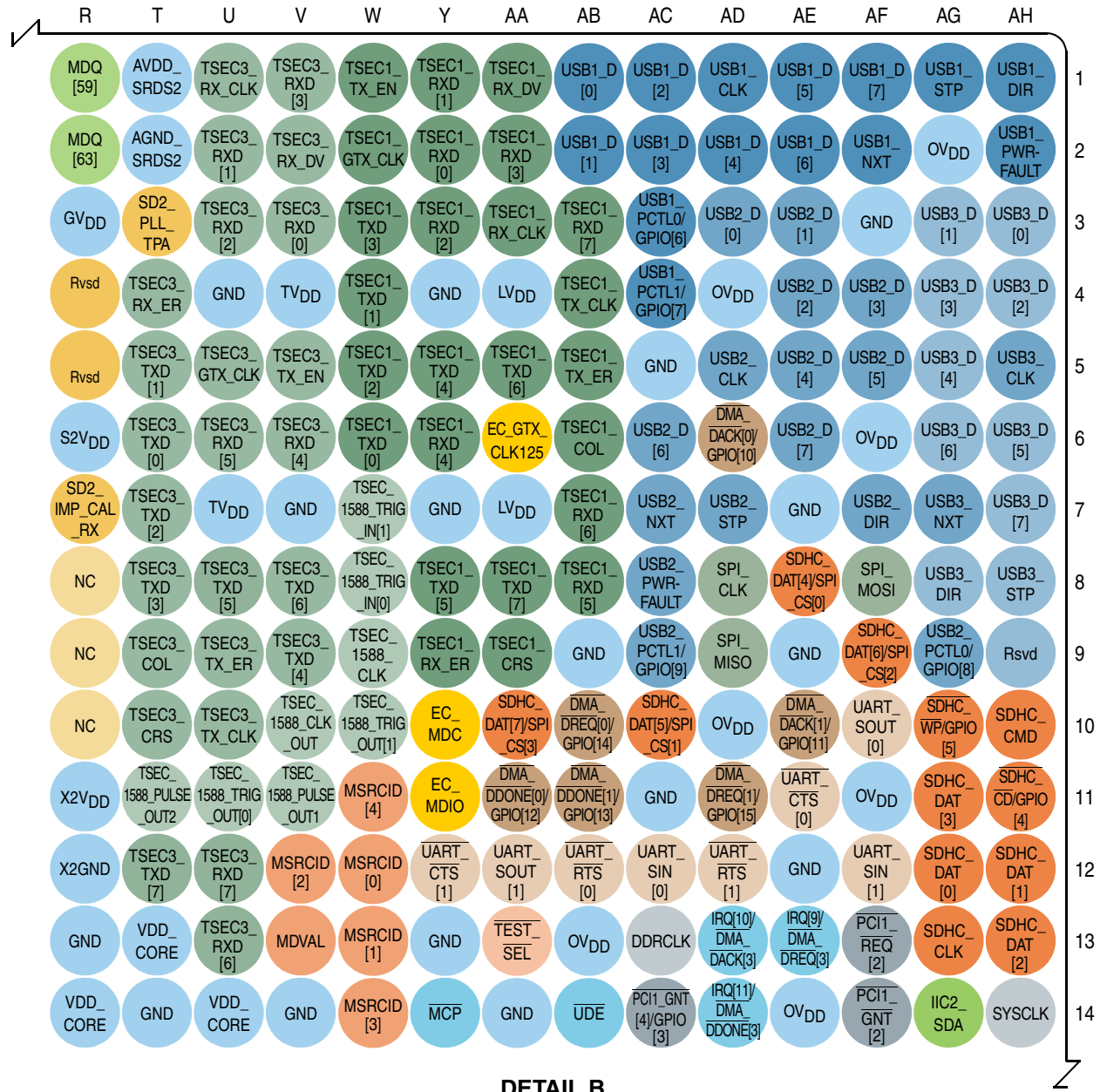
DETAIL B
