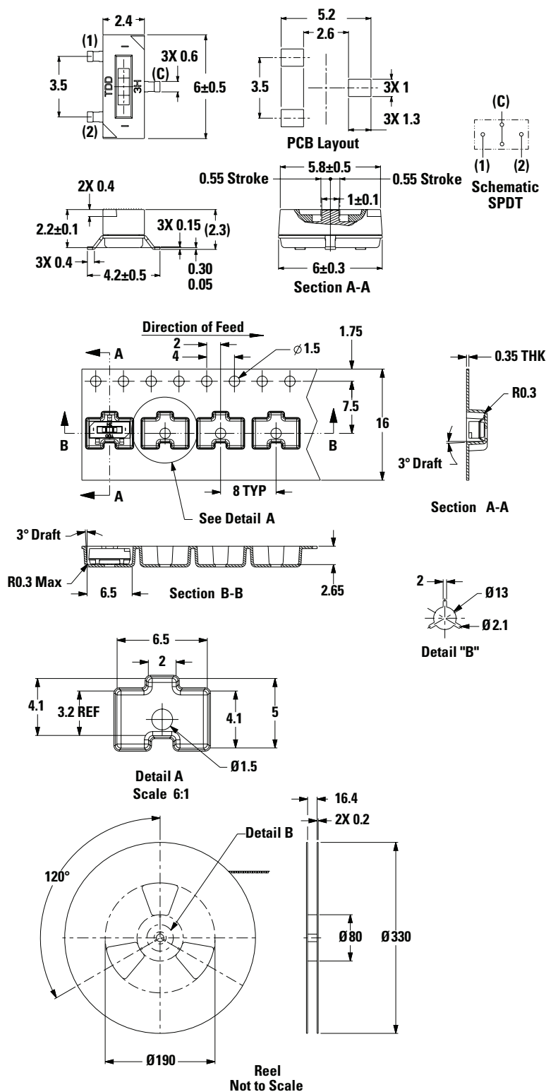
TDD Series Drawing and Dimensions (mm)
