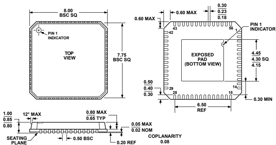
COMPLIANT TO JEDEC STANDARDS MO-220-VLLD-2 Figure 52. 56-Lead Lead Frame Chip Scale Package [LFCSP_VQ] 8 mm × 8 mm Body, Very Thin Quad (CP-56-2) Dimensions shown in millimeters
