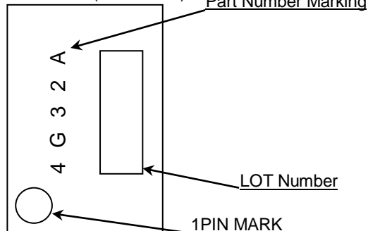
TSSOP-B8(TOP VIEW)
