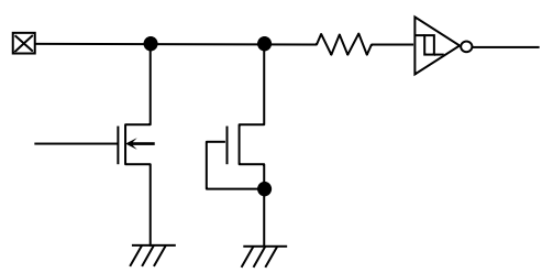
Figure 51. Input / Output Pin Circuit Diagram
