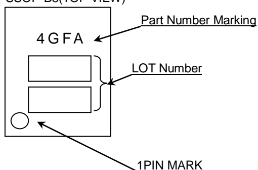
SSOP-B8(TOP VIEW)
