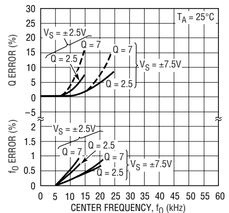
Mode 3, ( f_{CLK}/f_0 ) = 50:1
