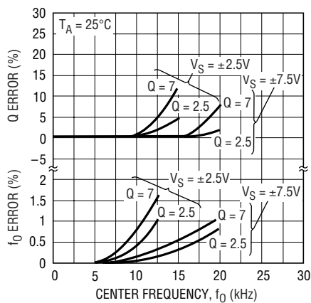
Mode 1, ( f_{CLK}/f_0 ) = 100:1
