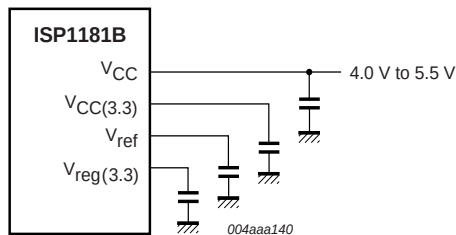
Fig 9. ISP1181B with a 4.0 V to 5.5 V supply.
