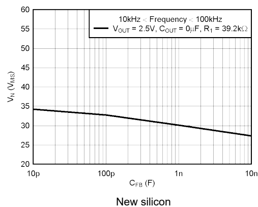
Figure 5-48. TPS73201 RMS Noise Voltage vs C_{FB}
