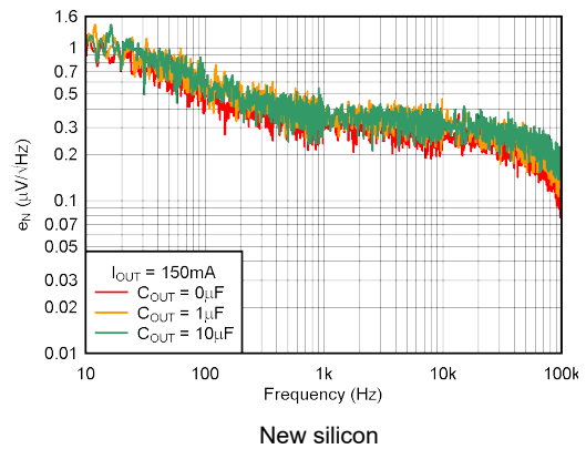
Figure 5-28. Noise Spectral Density C_{OUT} = 0\mu\text{F}
