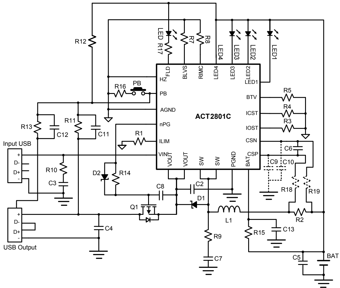
Figure 23. Typical application circuit (Input current limit 2.0A, fast charge current limit 1.5A, boost output constant current limit 1.3A)
