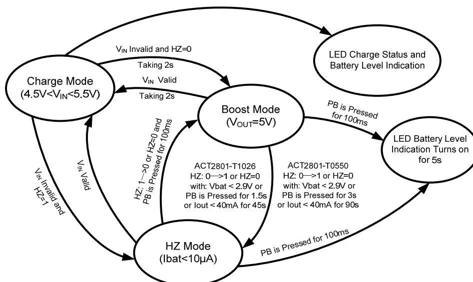
ACT2801 System Operation Flow Chart
