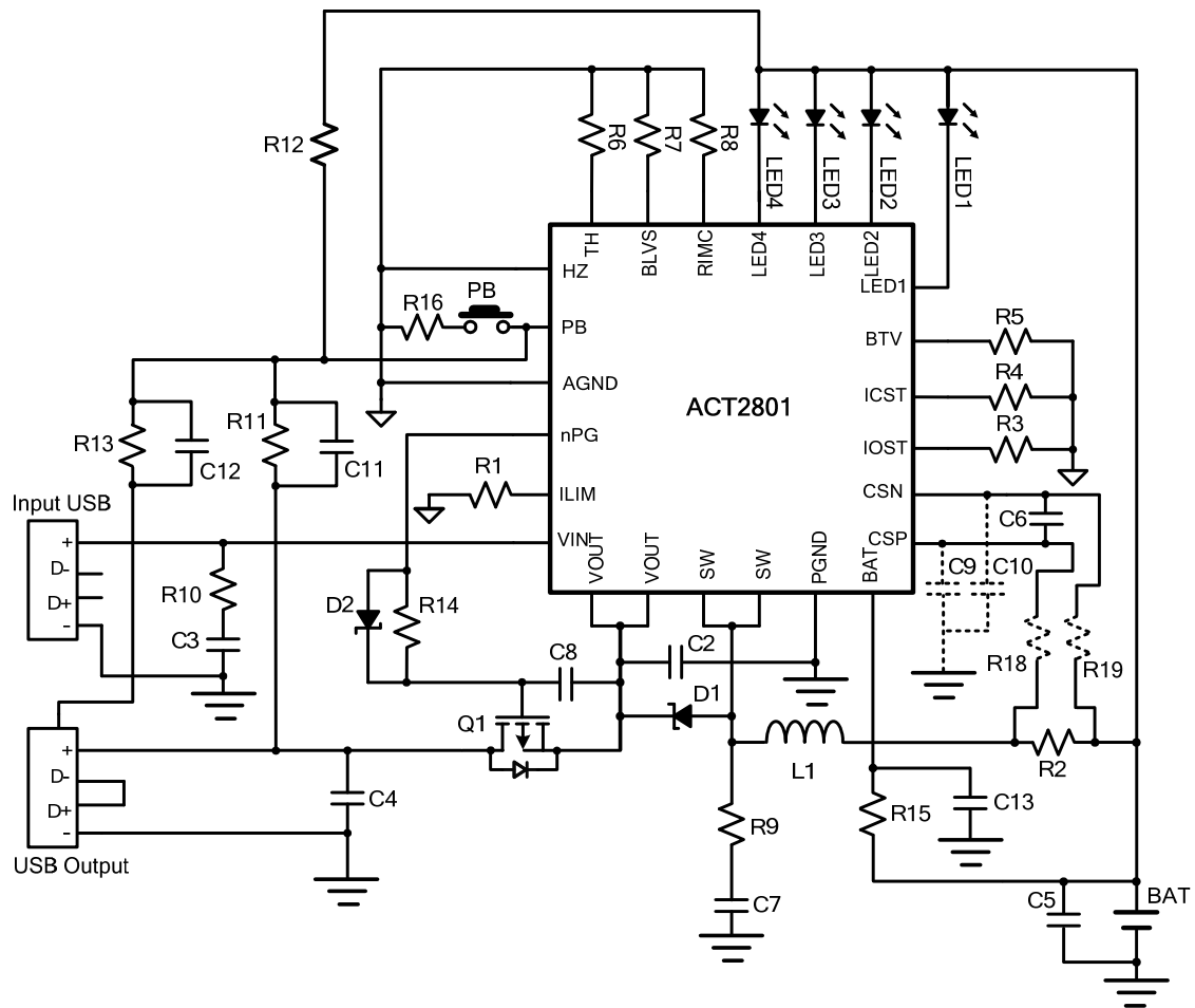
Figure 22. Typical application circuit (Input current limit 2.0A, fast charge current limit 1.5A, boost output constant current limit 1.3A)
