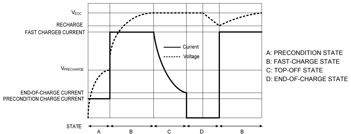
Typical Li+ Charge Profile and ACT2801/ACT2801C Charge States
