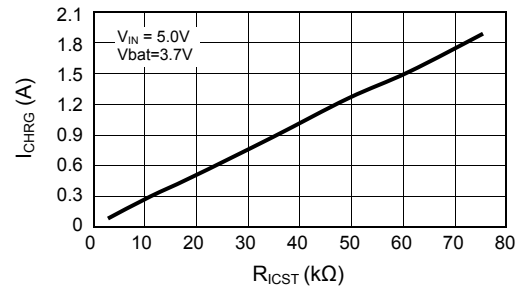
Figure 11. Battery fast charge current setting
