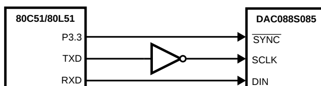
Figure 42. 80C51/80L51 Interface
