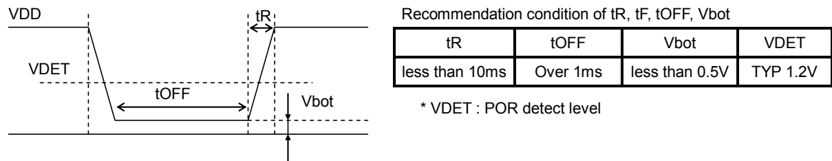
Figure 21. Power ON/OFF waveform
