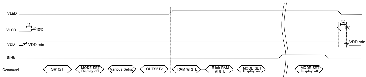
Figure 25. LED power supply On/Off sequence
