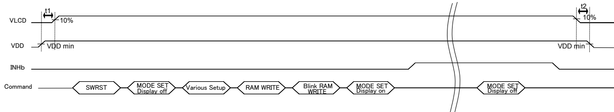
Figure 23. Power On/Off Sequence
