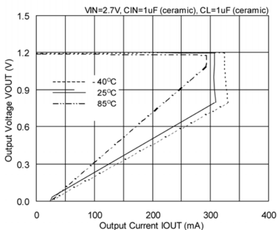
XC6209B122
