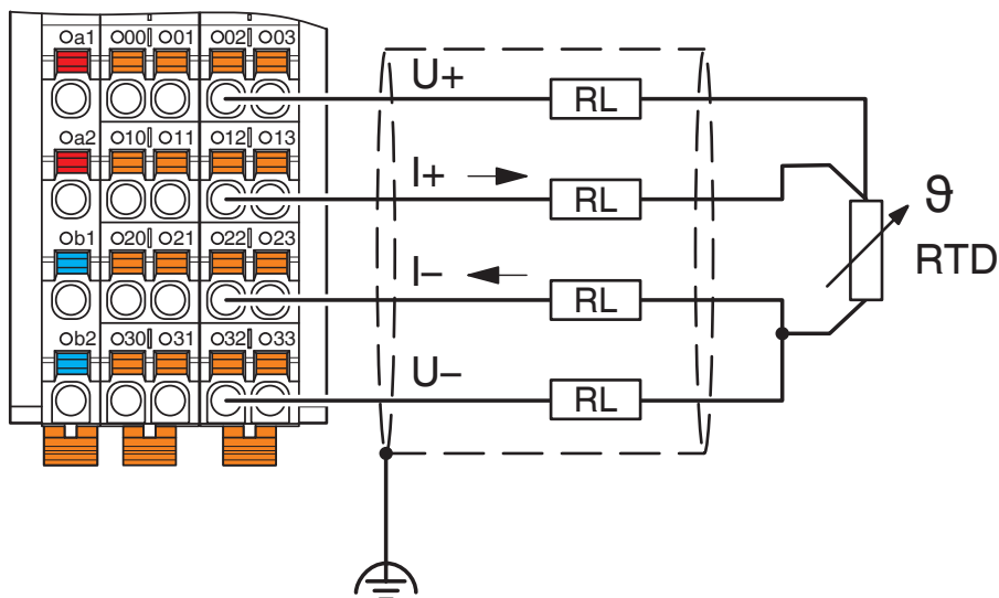
Connection diagram
