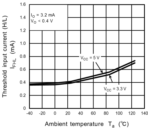
Fig. 13.2.9 I_{FHL} - T_a
