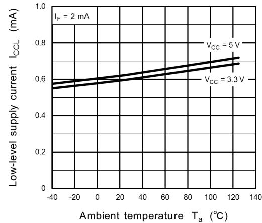
Fig. 13.2.7 I_{CCL} - T_a
