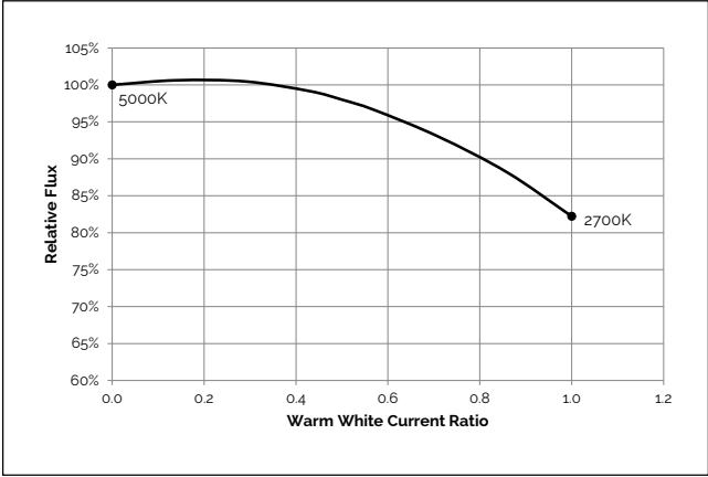
Figure 7: Relative Flux vs. Warm White Current Ratio
