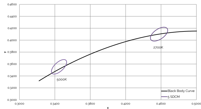
Figure 13: Graph of Bins in xy Color Space
