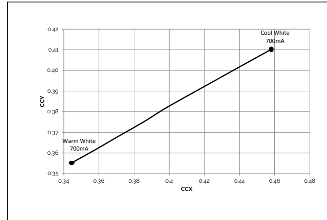
Figure 6: Color shift vs. Forward Current
