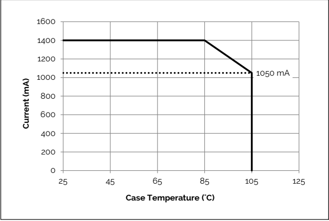
Figure 8: Derating Curve
