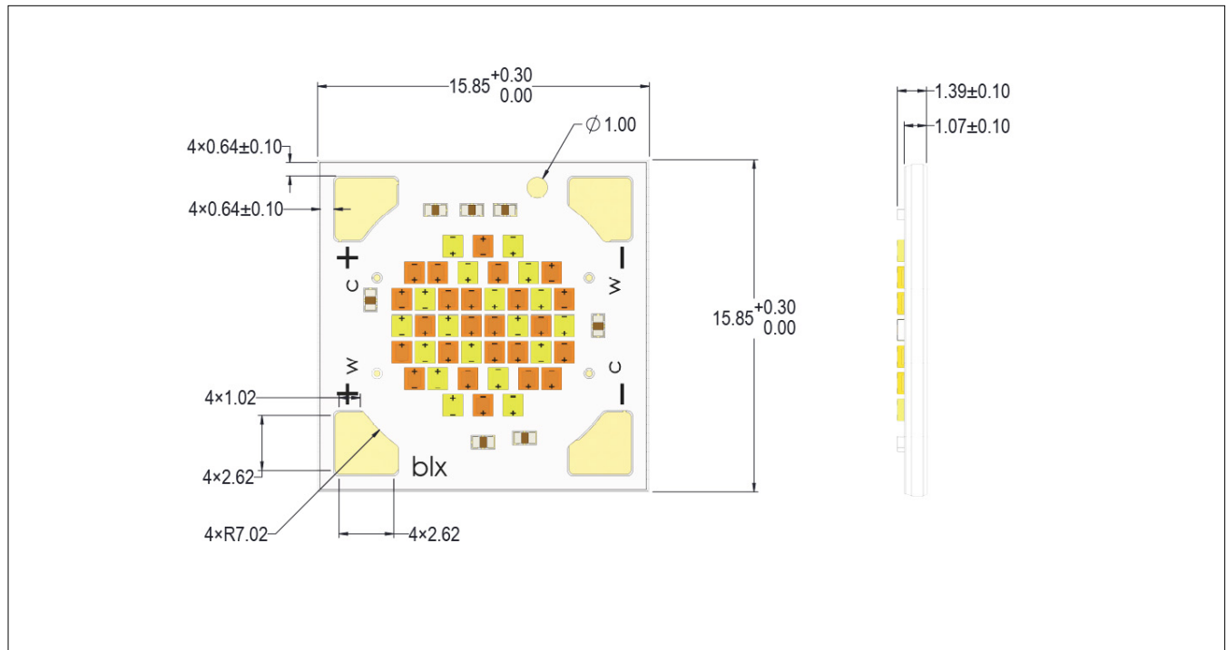
Figure 12: Drawing for Vesta Series Tunable White gmm Array
