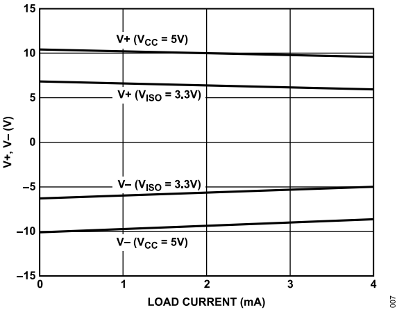
Figure 8. Charge Pump V + , V - vs. Load Current
