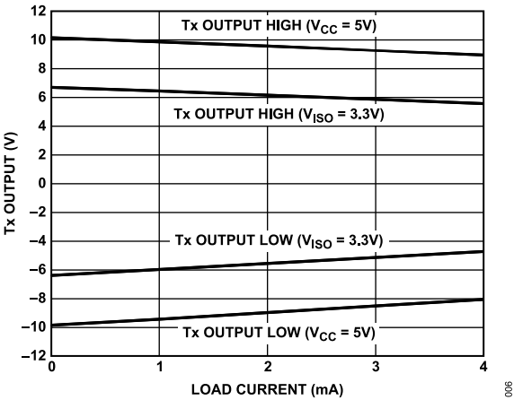
Figure 7. Transmitter Output Voltage High/Low vs. Load Current
