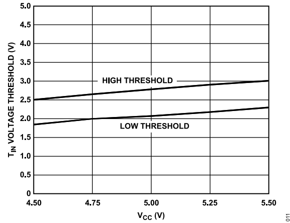
Figure 13. T_{IN} Voltage Threshold vs. V_{CC}
