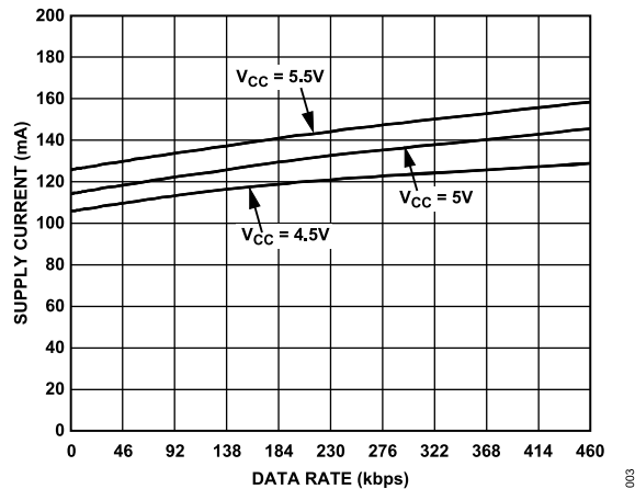
Figure 11. Primary Supply Current vs. Data Rate
