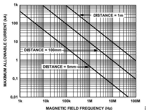
Figure 21. Maximum Allowable Current for Various Current-to-ADM3251E Spacings
