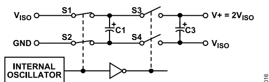
Figure 17. Charge Pump Voltage Doubler
