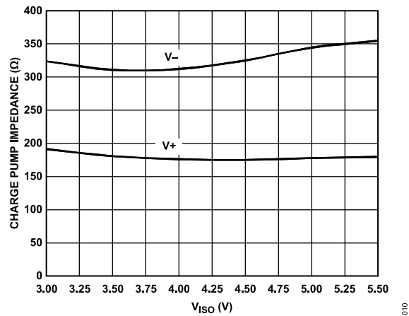
Figure 10. Charge Pump Impedance vs. V_{ISO}
