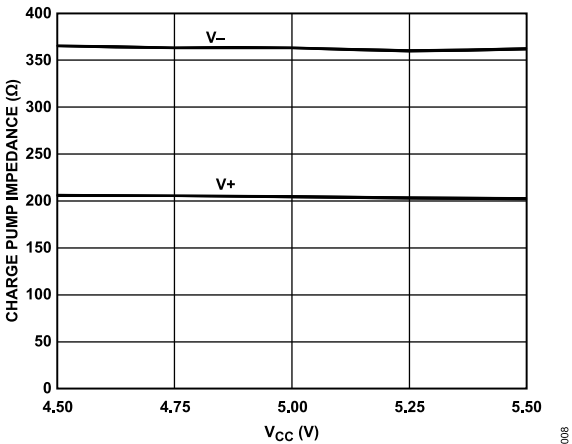
Figure 9. Charge Pump Impedance vs. V CC
