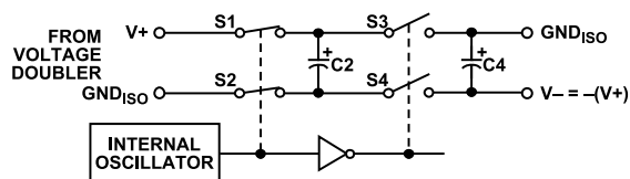
Figure 18. Charge Pump Voltage Inverter
