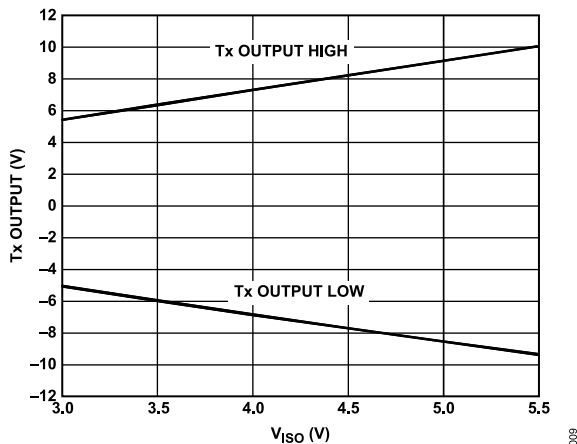
Figure 6. Transmitter Output Voltage High/Low vs. V ISO , R L = 3kΩ
