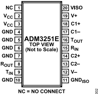
Figure 3. Pin Configuration
