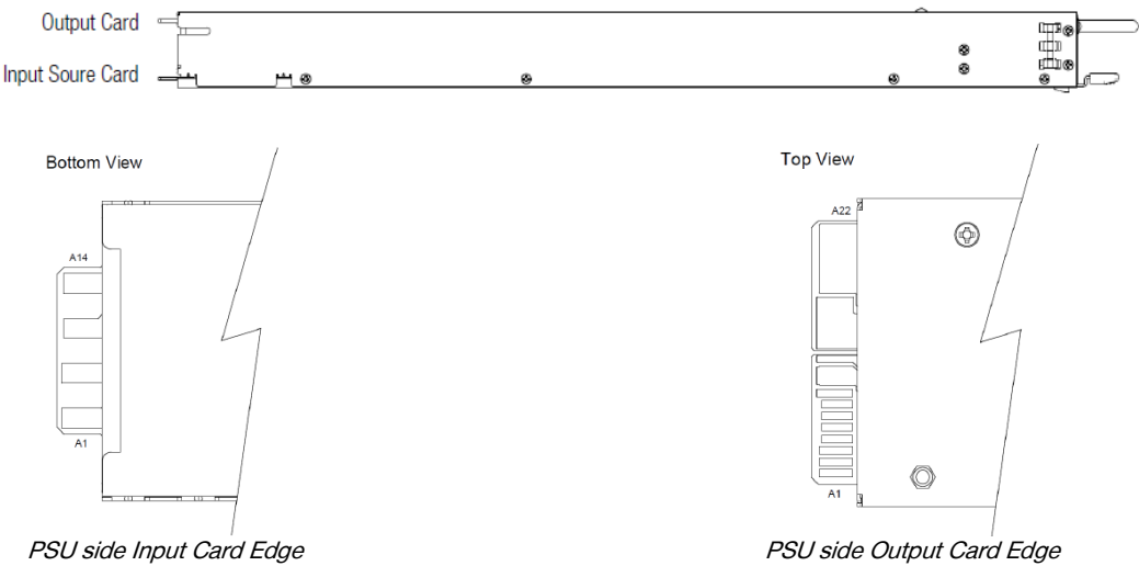
Figure 14. PSU rear side gold fingers
