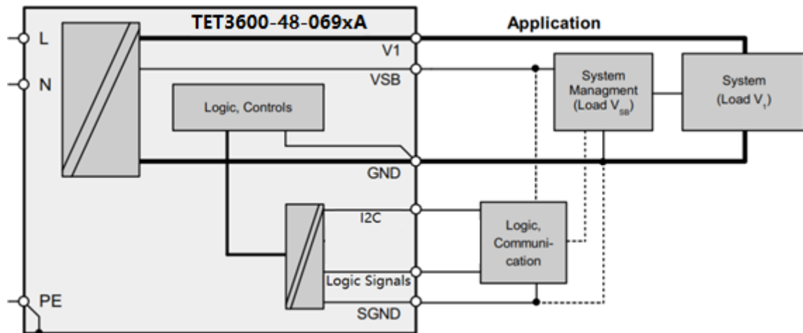
Figure 4. Output connection
