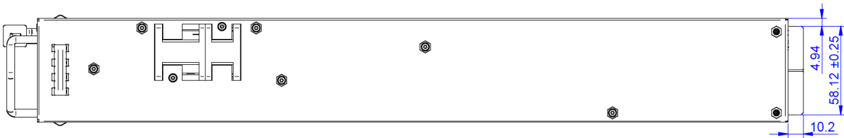
Figure 12. Bottom view
