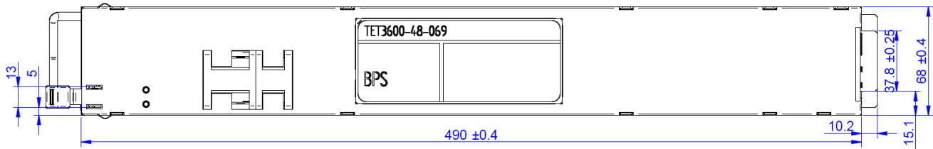
Figure 10. Top view
