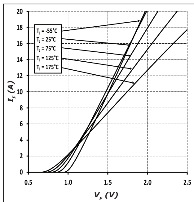
Figure 1. Forward Characteristics
