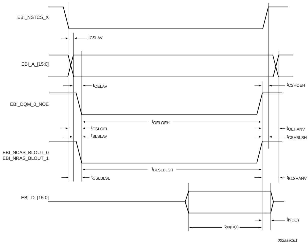
Fig 14. External memory read access to static memory
