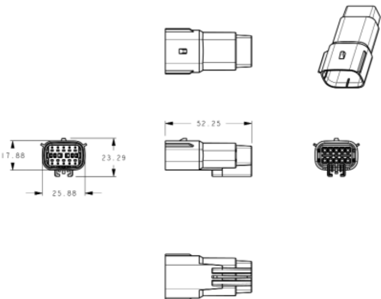
Male connector
