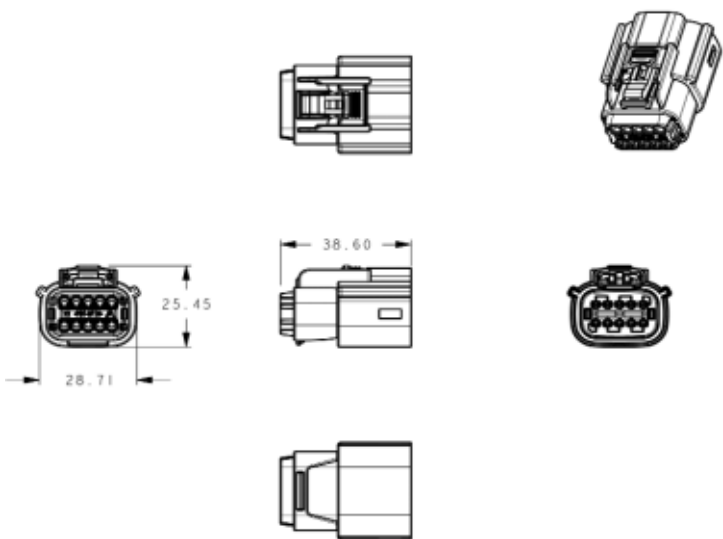
Female connector
