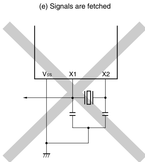
Figure 5-7. Examples of Incorrect Resonator Connection (2/2)
