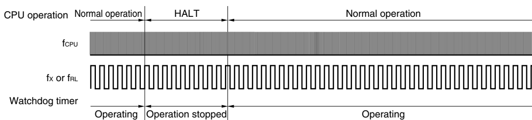
Figure 8-8. Operation in HALT Mode
