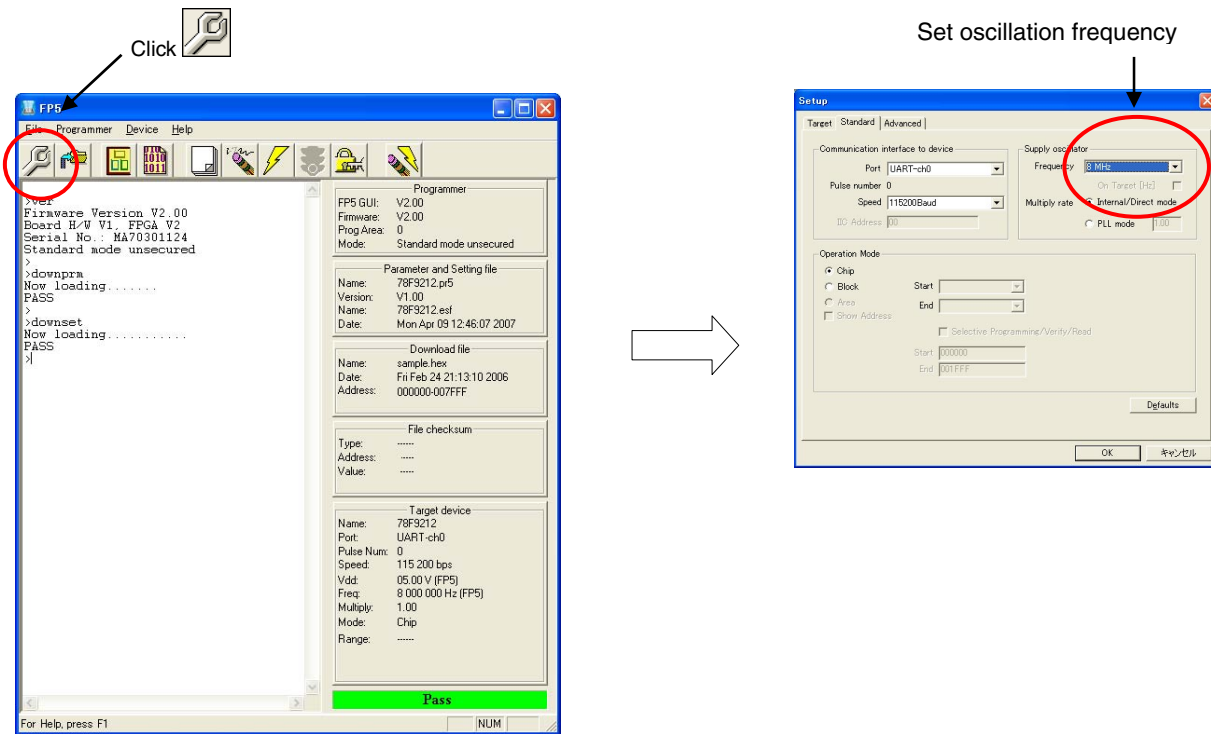
Figure 16-5. PG-FP5 Programming GUI Setting Example
