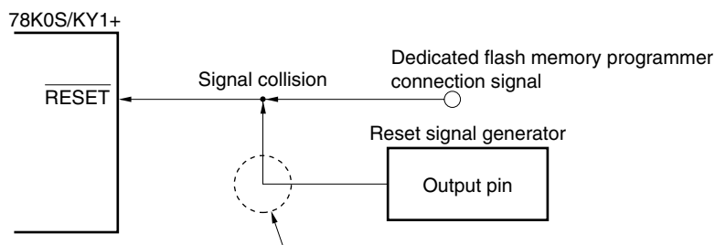
Figure 16-6. Signal Collision ( \overline{\text{RESET}} Pin)
