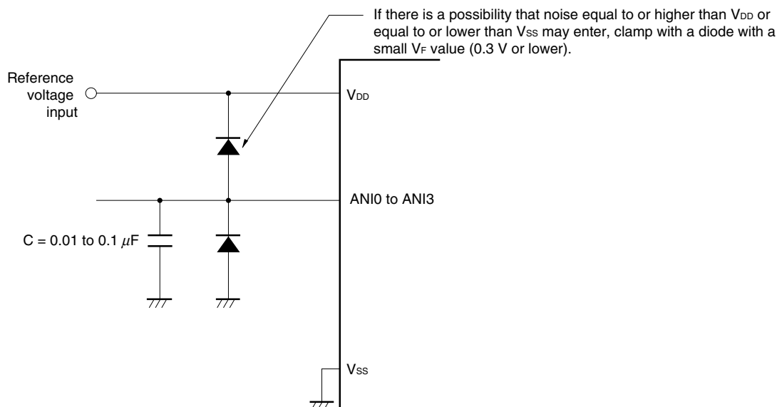
Figure 9-19. Analog Input Pin Connection
