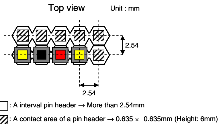
Figure B-2. When using the 78K0S/Kx1+ target cable (single track)
