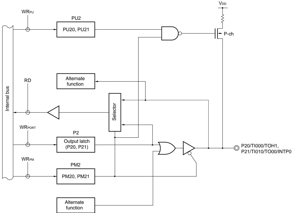
Figure 4-2. Block Diagram of P20 and P21 (2/2)
