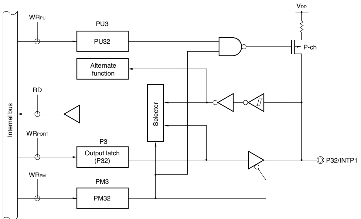
Figure 4-5. Block Diagram of P32
