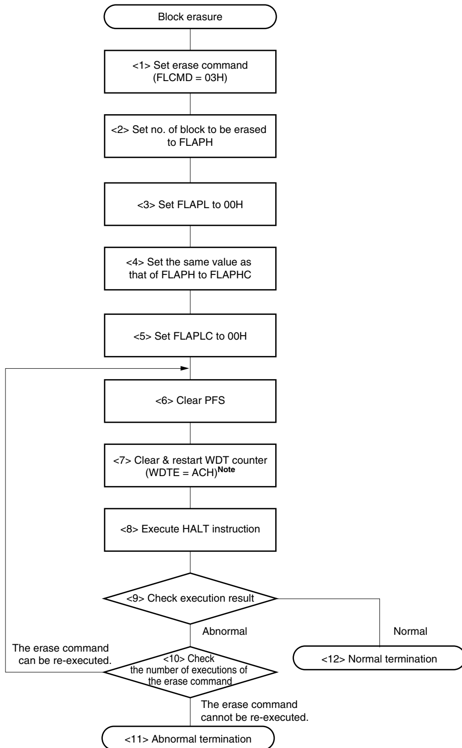
<R> Figure 16-20. Example of Block Erase Operation in Self Programming Mode
