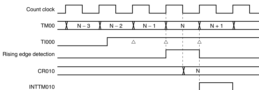
Figure 6-18. CR010 Capture Operation with Rising Edge Specified
