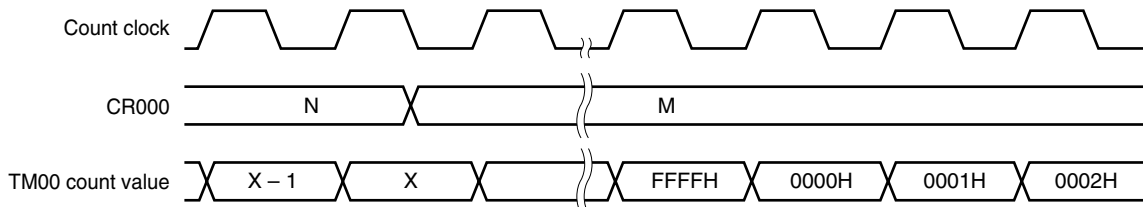
Figure 6-14. Timing After Change of Compare Register During Timer Count Operation (N → M: N > M)
