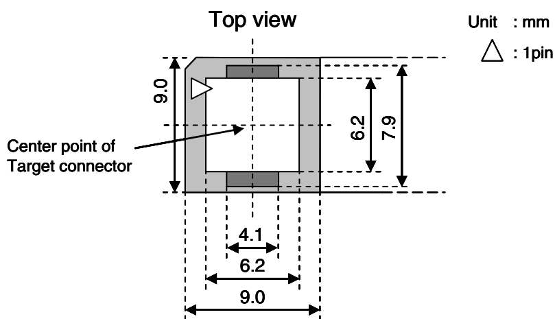
Figure B-1. When using the 78K0S/Kx1+ emulation probe (For 16-Pin GR Package)
