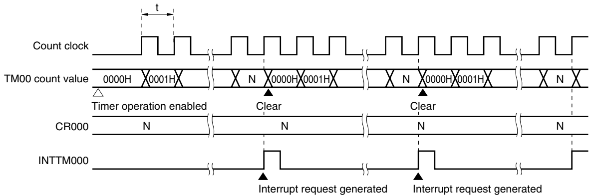
Figure 6-13. Timing of Interval Timer Operation
