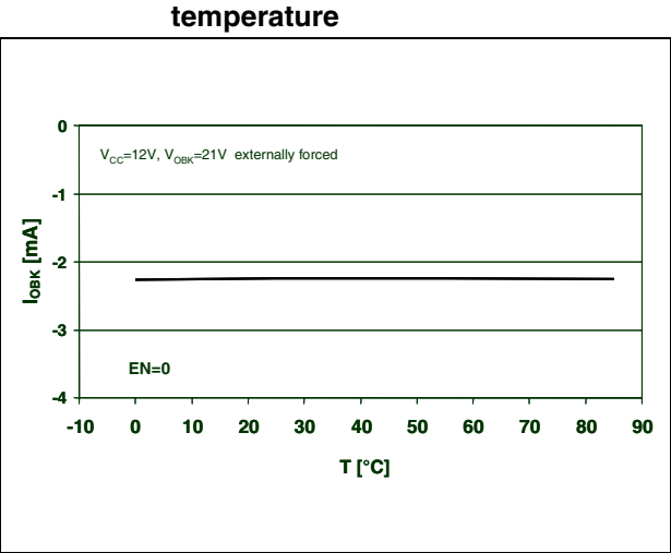
Figure 25. Output backward current vs. temperature
