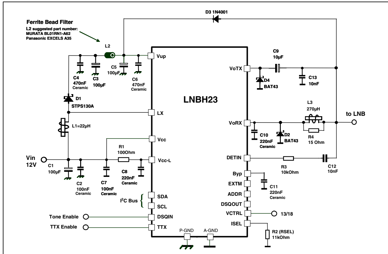
Component Notes R1, R4 1/4W resistors. Refer to the typical application circuit for the relative values R2 (RSEL), R3 1/4W resistors. Refer to the typical application circuit for the relative values C1 25V electrolytic capacitor, 100μF or higher is suitable. C9 10μF, >35V electrolytic capacitor C3, C5 100μF, >25V electrolytic capacitor, ESR in the 150mΩ to 350mΩ range C2, C4, C6, C7, C8, C10, C11, C12, C13 >25V ceramic capacitors. Refer to the typ. appl. circuit for the relative values D1 STPS130A or any similar schottky diode with V_{RRM} > 25V and I_{F(AV)} higher than: I_{F(AV)} > I_{OUT\_MAX} \times (V_{UP\_MAX}/V_{IN\_MIN}) D2, D4 BAT43, 1N5818, or any schottky diode with I_{F(AV)} > 0.2A , V_{RRM} > 25 V , V_F < 0.5 V D3 1N4001 or equivalent L1 22 μH Inductor with I_{sat} > I_{peak} where I_{peak} is the boost converter peak current (see Equation 1 )
