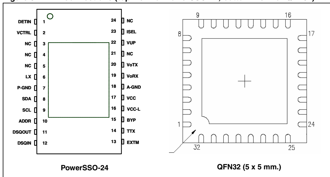
Figure 3. Pin connections (top view for PowerSSO-24, bottom view for QFN32)
