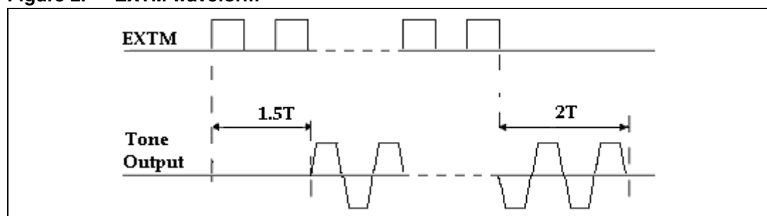
Figure 2. EXTM waveform
