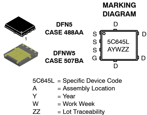
N-CHANNEL MOSFET
