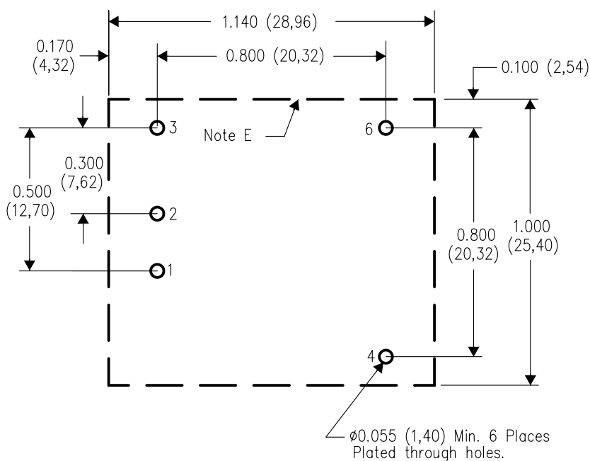
PC LAYOUT
