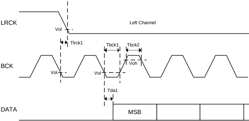
Figure 20. Output Timing
