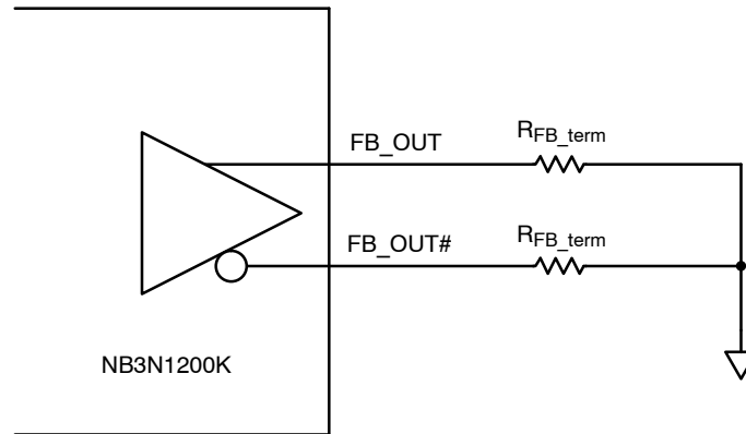
Figure 12. External Feedback Example Schematic
