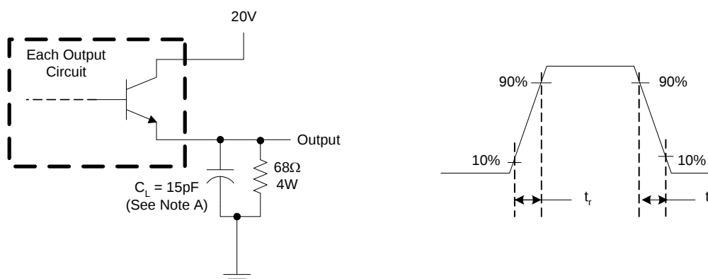
Figure 7. Emitter-Follower Configuration
