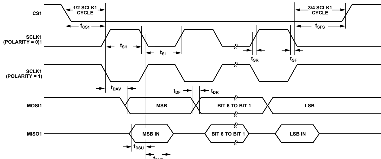
Figure 4. SPI Master Mode Timing (Phase Mode = 1)
