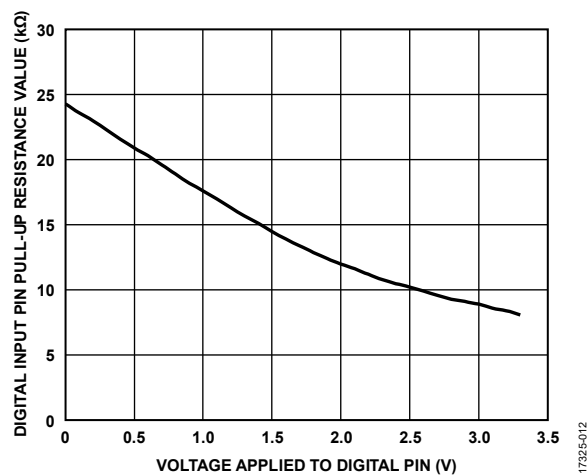
Figure 10. Digital Input Pin Pull-Up Resistance Value vs. Voltage Applied to Digital Pin, T_A = 25^\circ\text{C} , IOVDD = 3.4 V
