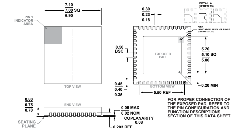
Figure 13. 48-Lead Lead Frame Chip Scale Package [LFCSP] 7 mm × 7 mm Body and 0.75 mm Package Height (CP-48-4)
