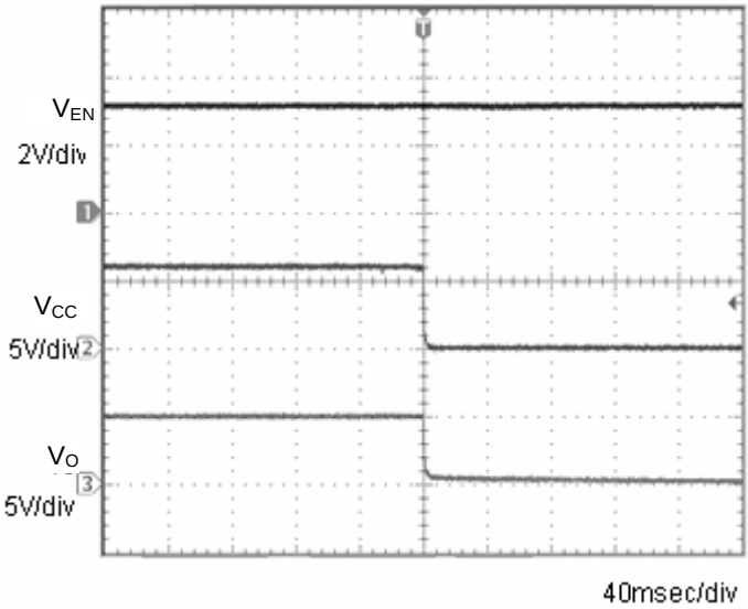
Fig.6 OFF sequence 1 Co=1µF
