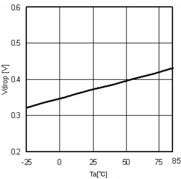
Fig.18 Minimum dropout Voltage ( V_{CC}=5\text{V} , I_O=-0.3\text{A} )
