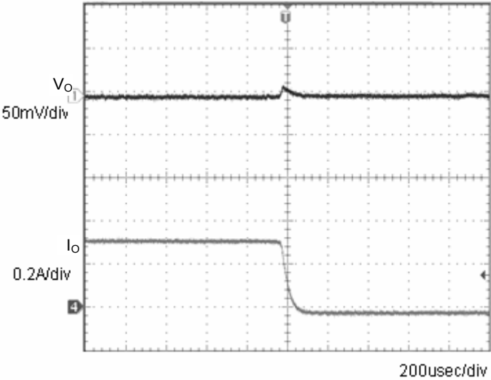
Fig.4 Transient Response (0.3→0A) Co=1µF
