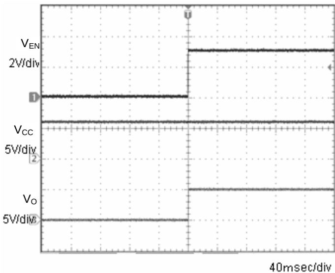
Fig.5 Input sequence 1 Co=1µF
