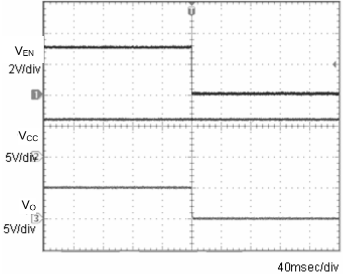
Fig.8 OFF sequence 2 Co=1μF
