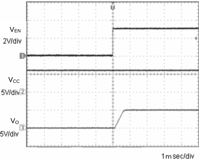
Fig.7 Input sequence 2 Co=1μF
