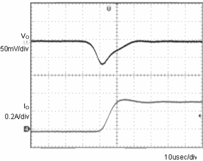
Fig.3 Transient Response (0→0.3A) Co=1µF
