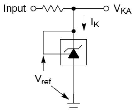
Figure 1: V_{KA} = V_{REF}
