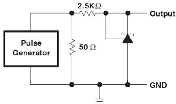
Test Circuit for Pulse Response, I_K = 1\text{ mA}
