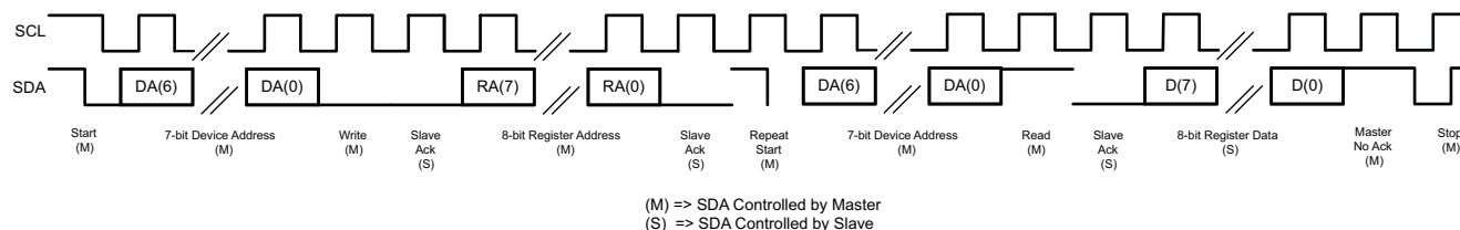
Figure 7-52. I²C Read
