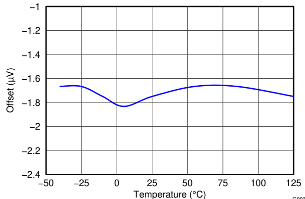
Figure 5-3. Shunt Input Offset Voltage vs Temperature
