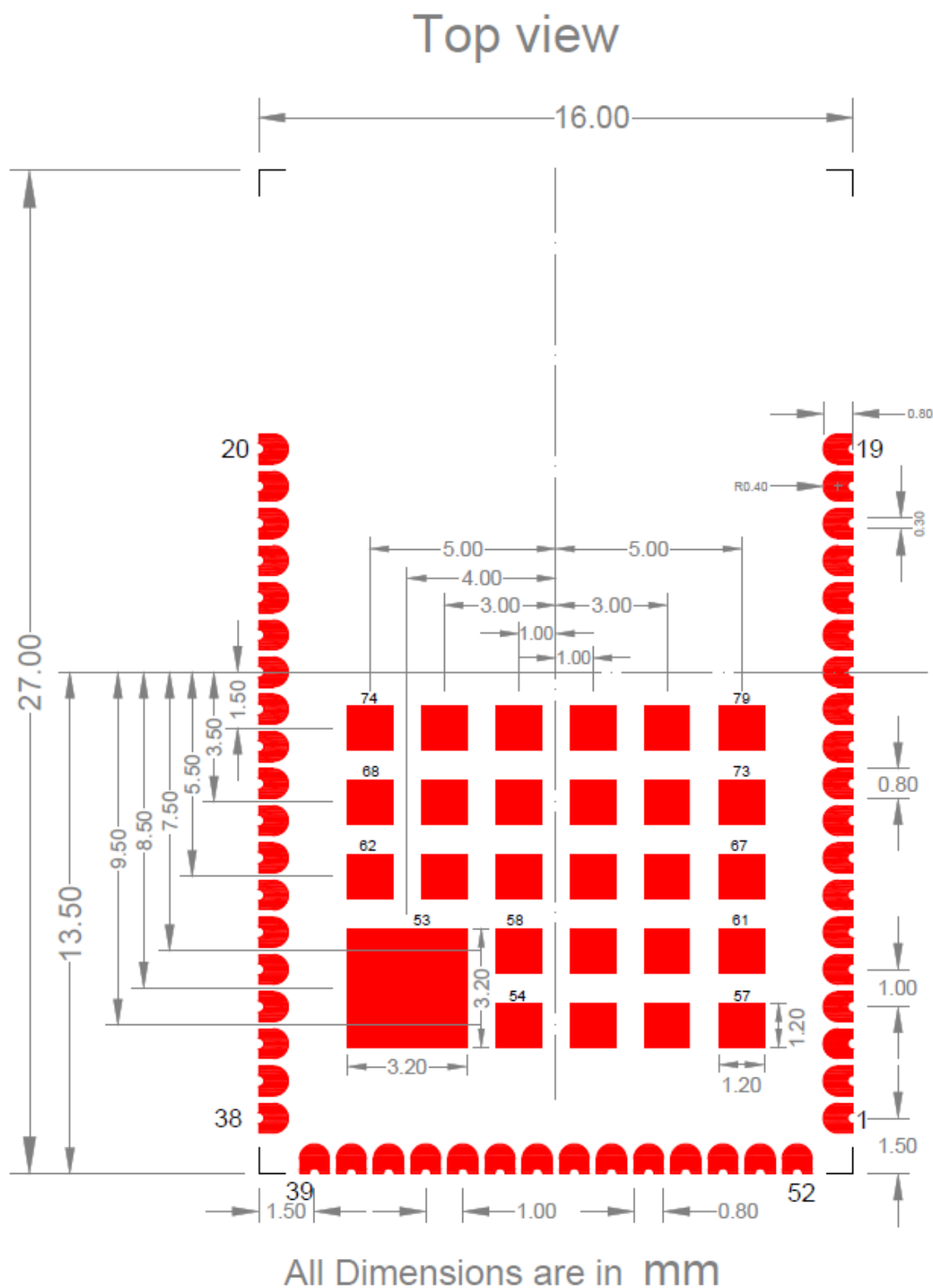
Figure 30. Package Outline
