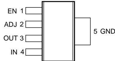
NDC Package (LP38692-ADJ only) 5-Pin SOT-223 Top View
