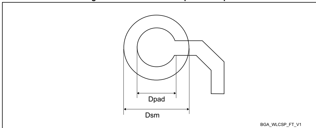
Figure 62. WLCSP39 - Footprint example
