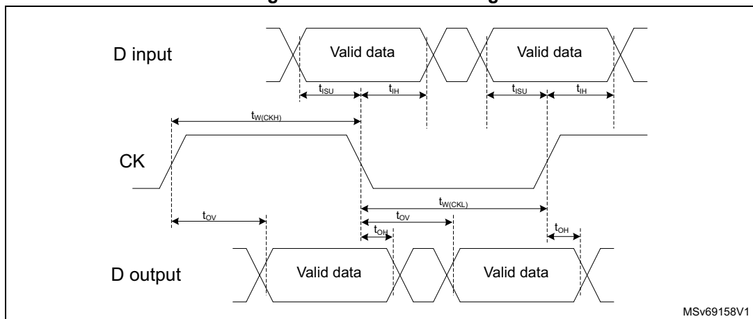
Figure 58. DDR mode timings
