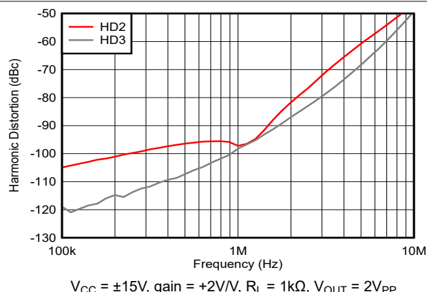
Figure 5-15. THS4031 Harmonic Distortion vs Frequency
