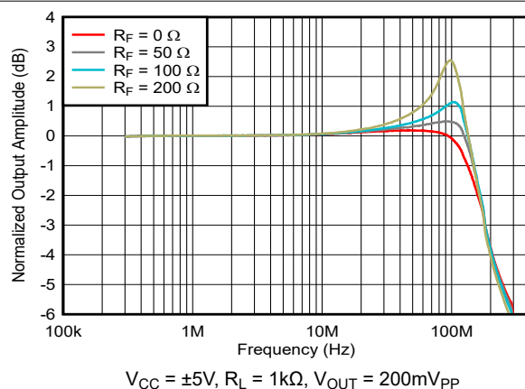
Figure 5-4. Frequency Response vs Feedback Resistance
