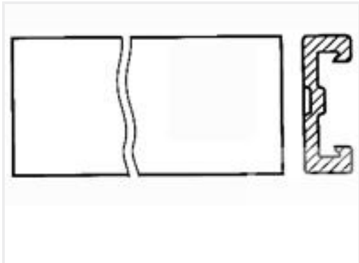
TE Part #1-640642-0 10P MTA100 COVER F/T
