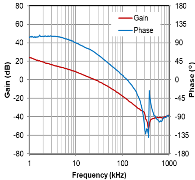
Figure 39. Frequency Characteristics ( V_{IN} = 12\text{ V} , I_{OUT} = 2\text{ A} )
