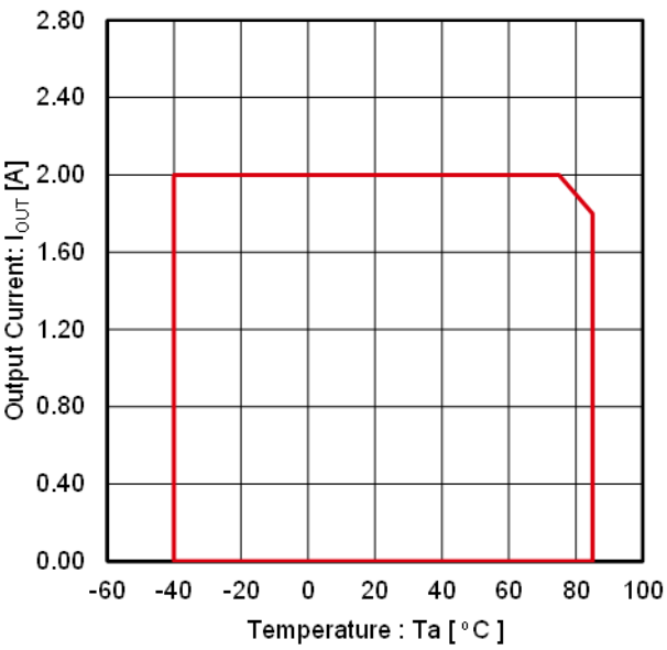
Figure 28. Output Current vs Temperature (Note 1) Operating Range: Tj < 150 °C (VIN = 12 V, 24 V, VOUT = 5 V)
