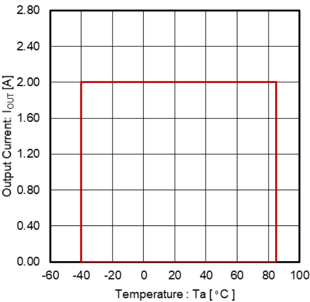
Figure 26. Output Current vs Temperature (Note 1) Operating Range: Tj < 150 °C (VIN = 5 V, 12 V, VOUT = 1.2 V)
