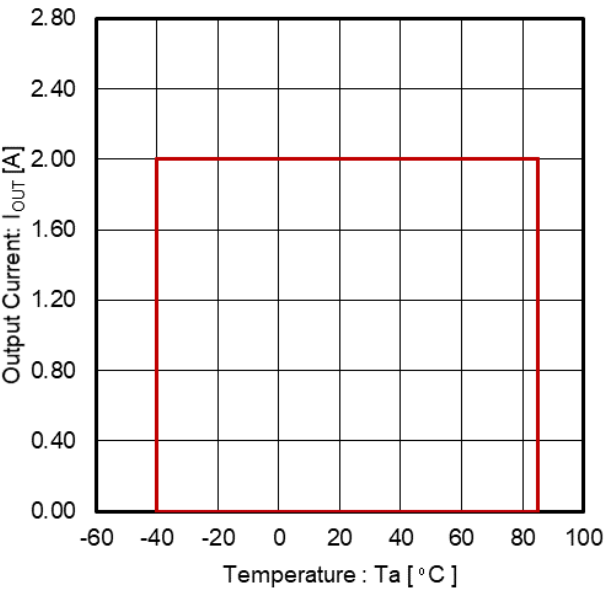
Figure 27. Output Current vs Temperature (Note 1) Operating Range: Tj < 150 °C (VIN = 12 V, 24 V, VOUT = 3.3 V)
