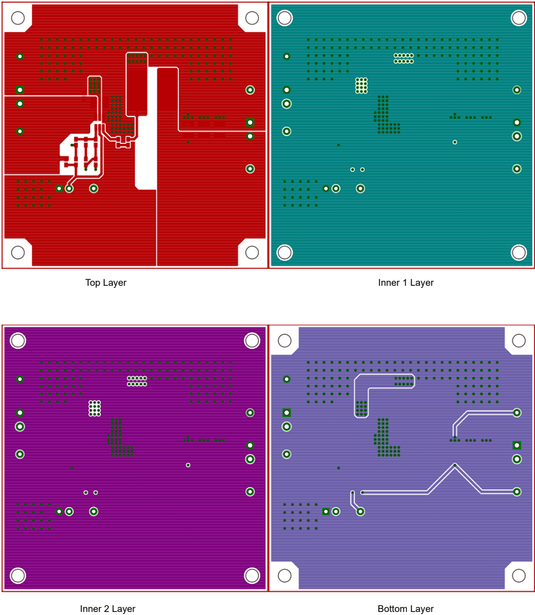
Figure 57. Example of PCB Layout
