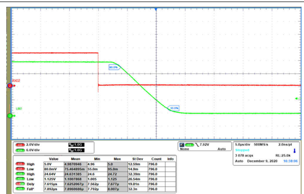
Figure 10-3. Recessive to Dominant Propagation
